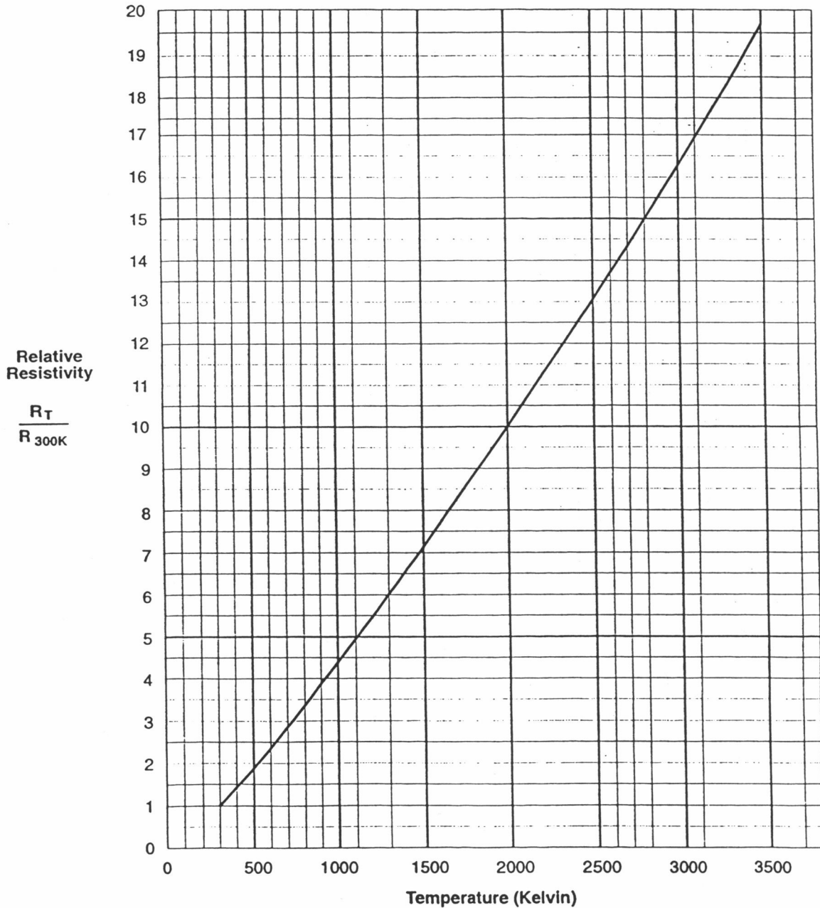
Temperature versus Resistivity for Tungsten
