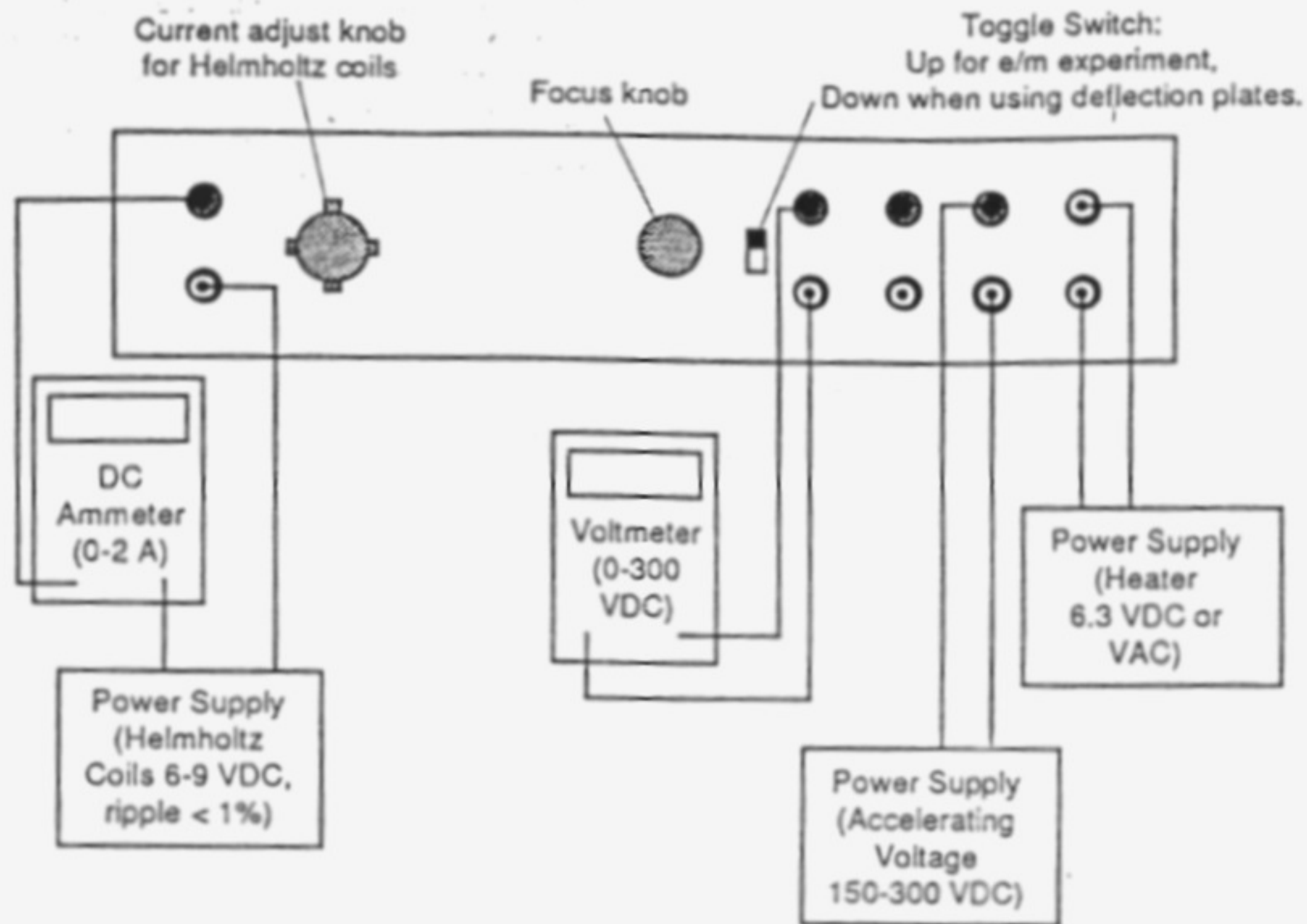
Connections for e/m Experiment
